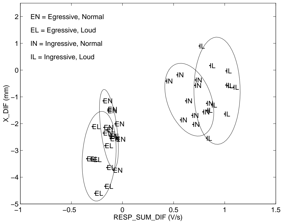
Tongue movement vs. respiratory activity. Subject M
