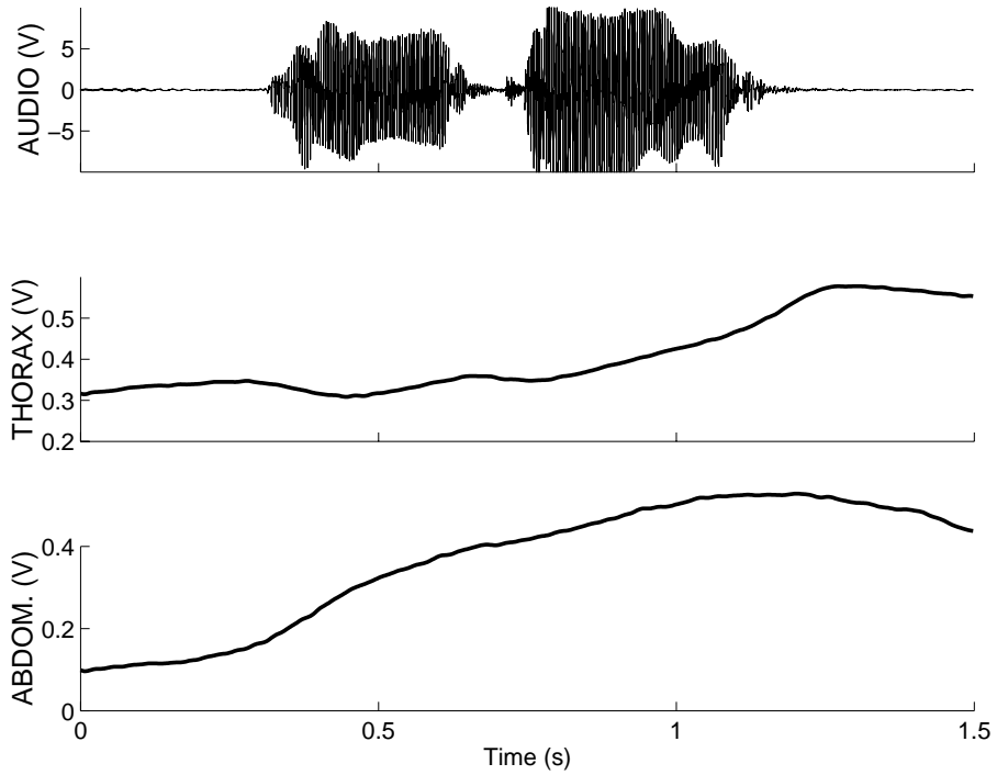
Speaker M, /ogo/, ingressive airflow, loud intensity
