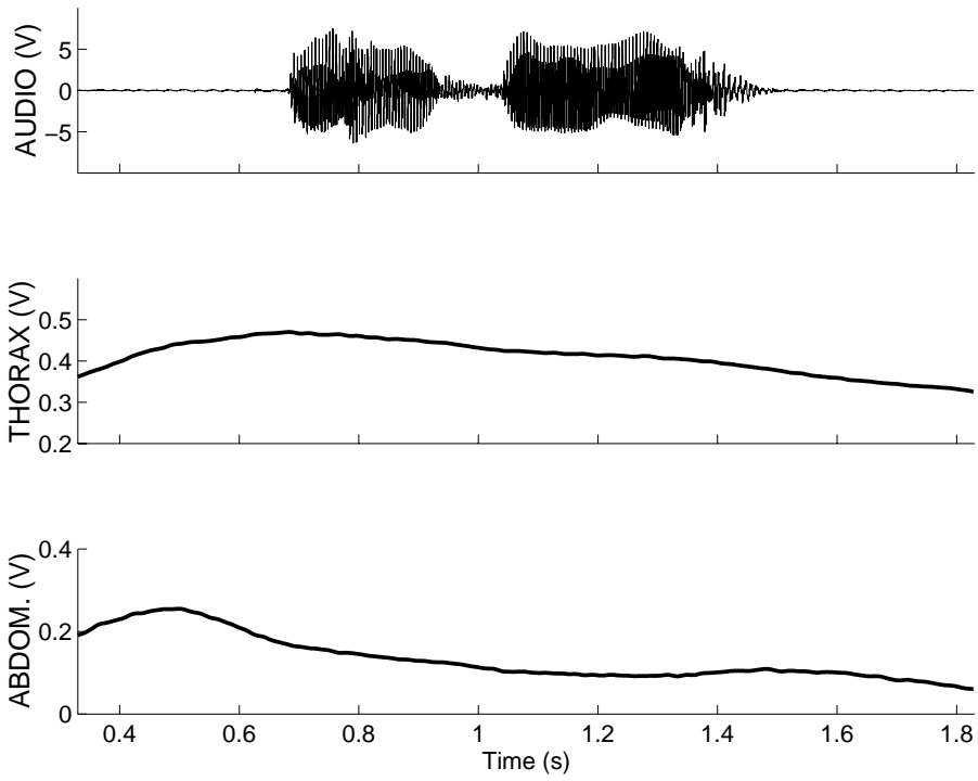
Speaker M, /ogo/, egressive airflow, loud intensity
