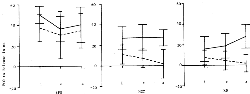
Fig. 1. Mean and sd for PGO to Release for the pre-stress stops; /p/ with unbroken line and with long horizontal bars delimiting the sd; /t/ with dashed line and with short bars.
