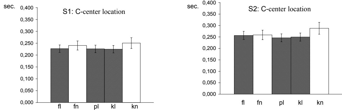
Fig. 3. Mean location of the C-center relative to the burst of the final stop; error bars show the standard deviation (time in sec.).
