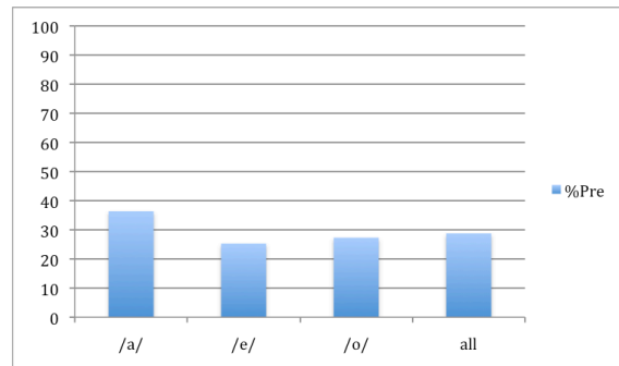
Figure 8. Frequency of preaspiration according to vowel type (values show the percentage of the 231 /a/, 356 /e/ and 348 /o/ tokens that were followed by a preaspiration).
