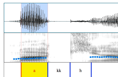
Figure 1. A voiceless velar stop /kk/ in macchina 'car' realised without preaspiration by a male speaker from Florence (LTp1A01F).
