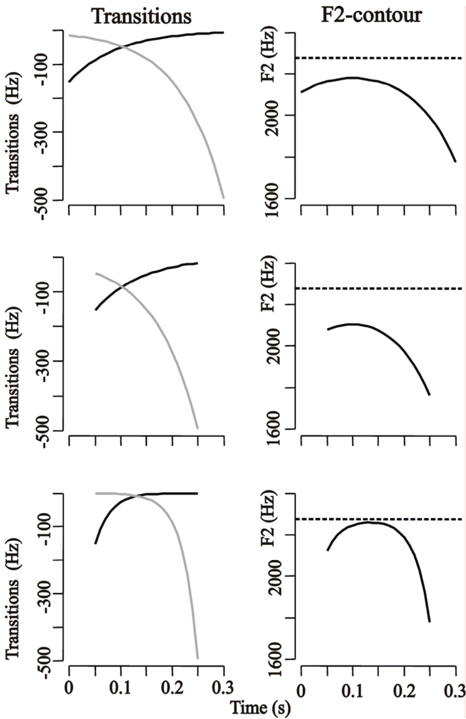
Fig. 5: An implementation of the equations (6) and (7) for constructing an F2-contour appropriate for the context [did] using the parameters given in Table VI of Broad & Clermont (1987). Left: the values of the initial [di] (black) and final [id] (gray) transitions. Right: the corresponding F2 contour that results when the transitions on the left are summed and added to the vowel target shown as horizontal dotted line. Row 1: vowel duration = 300 ms. Row 2: the same parameters are used as in row 1 but the duration is 100 ms less resulting in greater undershoot (shown as the extent by which the contour on the right falls short in frequency of the horizontal dotted line). Row 3: the same parameters as in row 2, except that the transition rates, defined by \beta in equations in (6) and (7), are faster.
