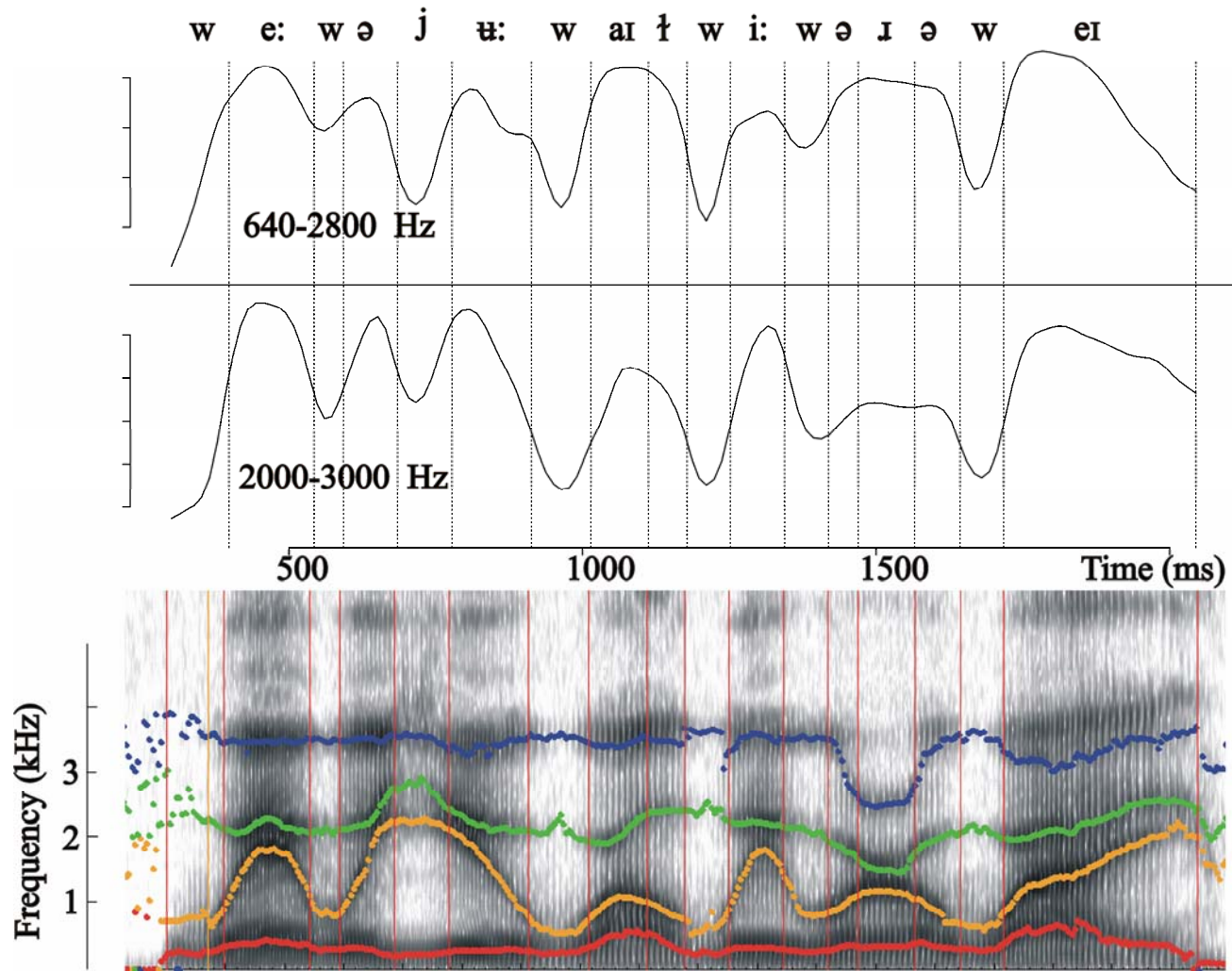
Fig. 9. Summed energy values in two frequency bands and the first four formant frequencies superimposed on a spectrogram of the sonorant-rich sentence 'where were you while we were away?' produced by an adult male, Australian English speaker. (Adapted from Harrington & Cassidy, 1999)
