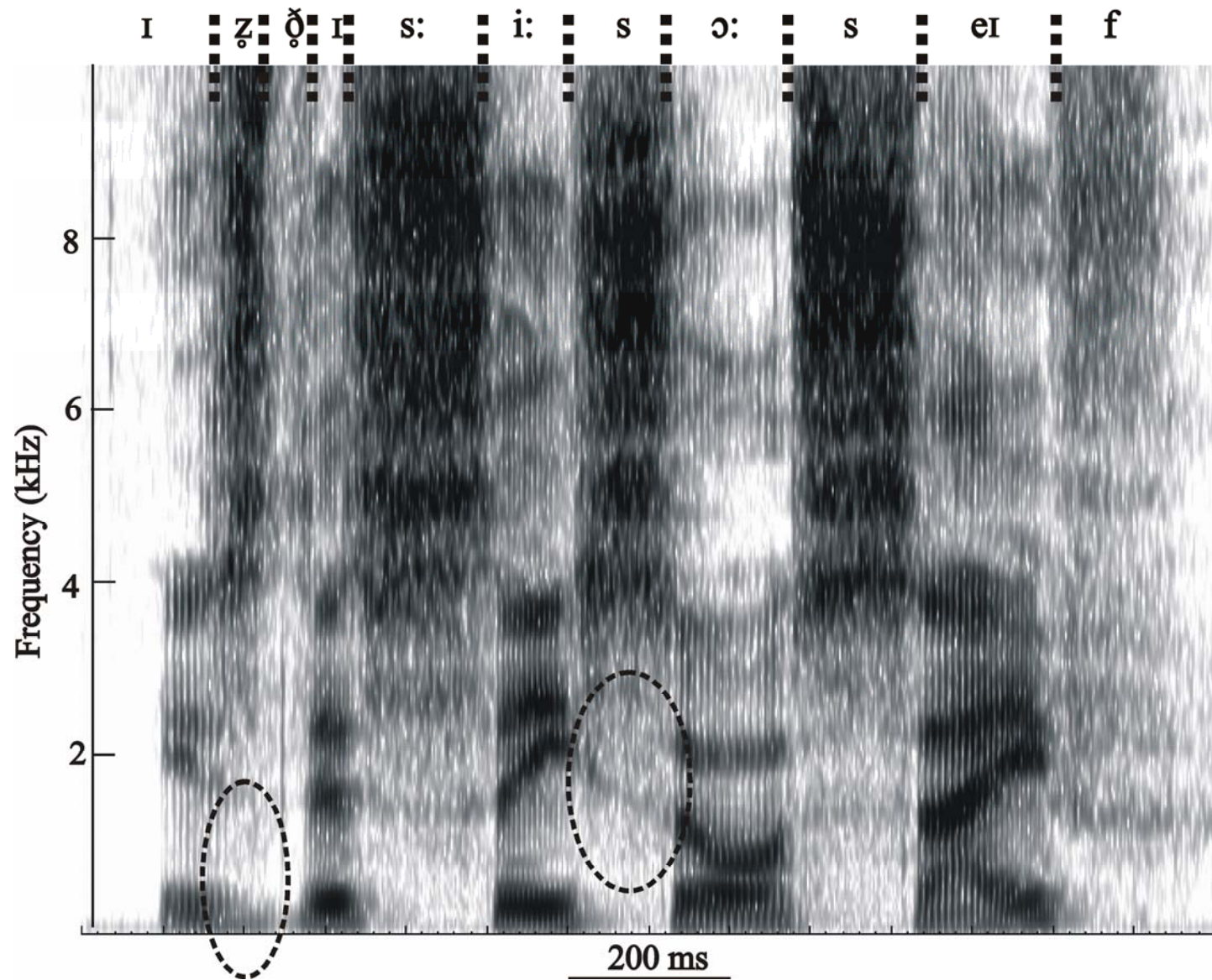
Fig. 10. Spectrogram of the sentence 'is this seesaw safe?' produced by an adult male speaker of Australian English. There is evidence of weak periodicity in the devoiced [z̥ʔ] at the boundary of 'is this' (ellipse, left) and of an F2 transition in the noise of the second [s] of 'seesaw' (ellipse, right). (Adapted from Harrington & Cassidy, 1999).
