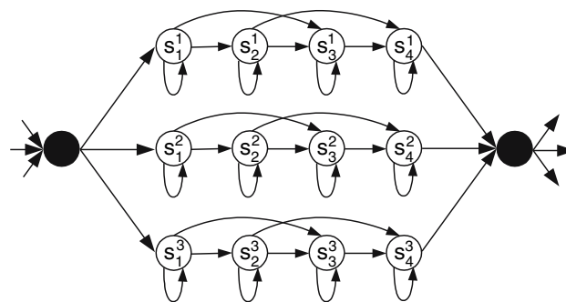
Fig. 43 Example PaHMM with three channels (Bakis topology)
