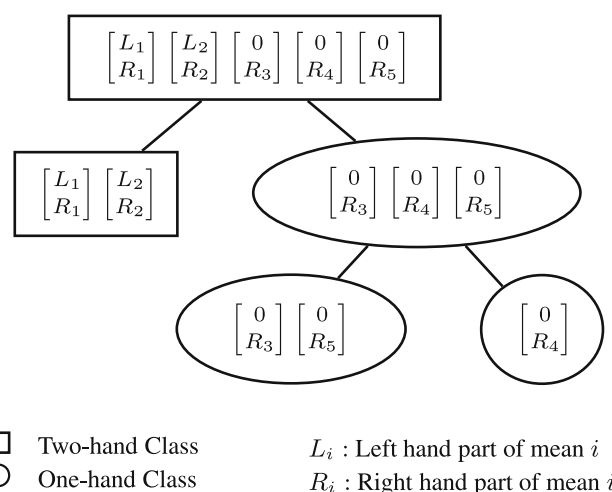
Fig. 49 One-hand classes as part of the regression class tree
