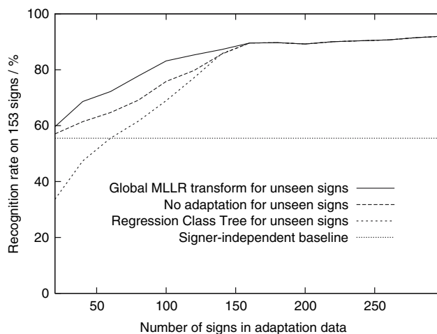
Fig. 51 Handling of unseen signs, supervised MLLR adaptation
