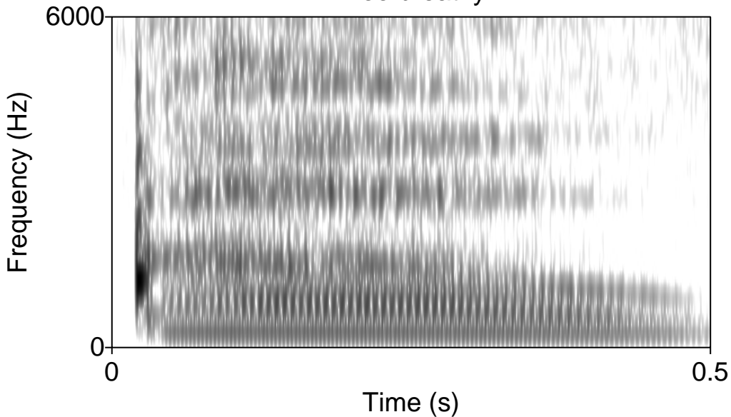
!Xoo breathy
