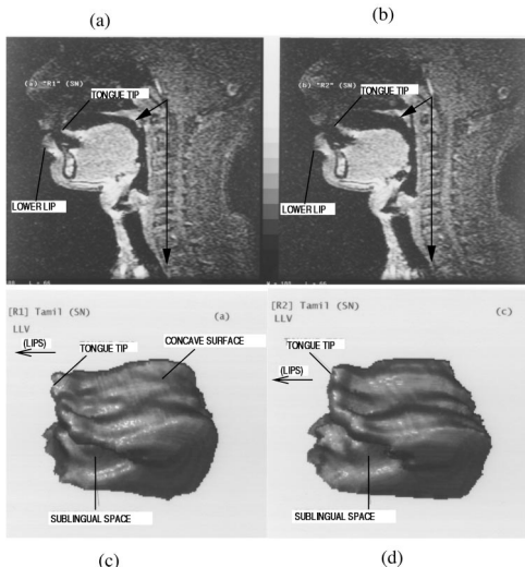
FIG. 2. (a) Midsagittal MR image for [r] . (b) Midsagittal MR image for [\underline{r}] . (c) 3-D tongue shape for [r] (tongue tip toward the left of panel). (d) 3-D tongue shape for [\underline{r}] (tongue tip toward the left of panel).
