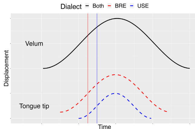
Fig. 13. A schematic outline of the displacement of the velum (black, for both dialects) and of the tongue tip (BRE: red dashed; USE: blue dashed) as a function of time. The vertical lines are the times of the peak velocity of tongue tip raising for BRE (red) and USE (blue). (For interpretation of the references to colour in this figure legend, the reader is referred to the web version of this article.)
