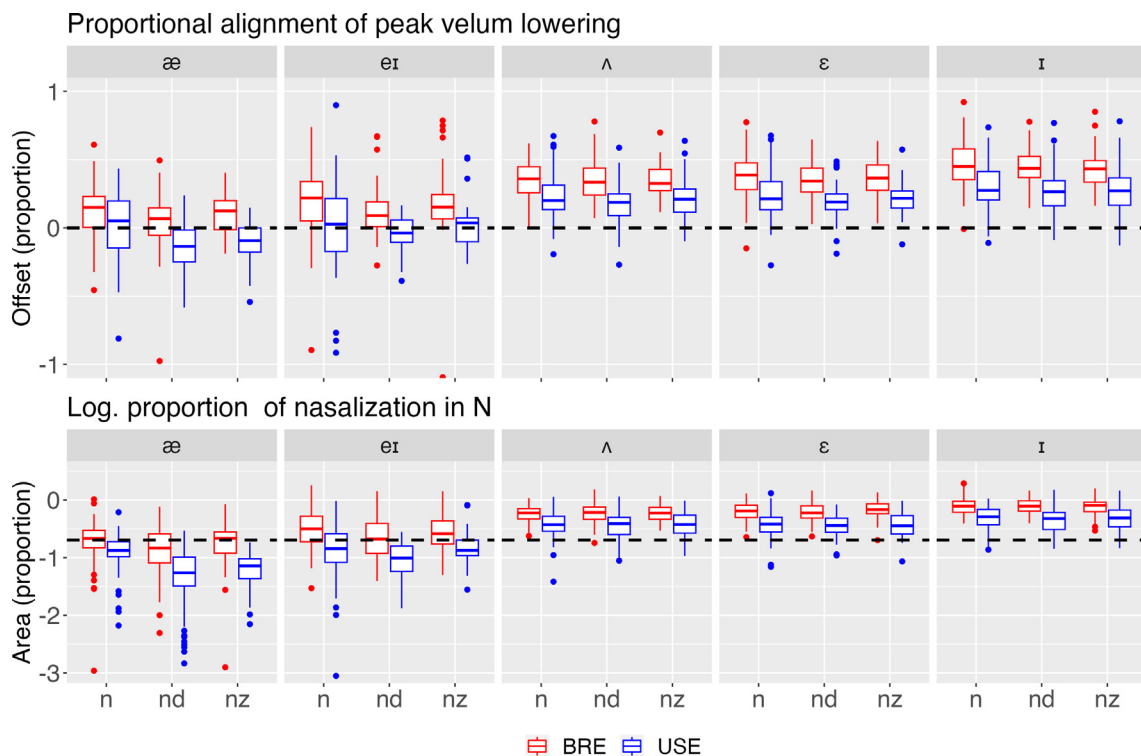
Fig. 3. Row 1: The proportional time of the peak velum lowering relative to the acoustic VN boundary ( i_1/i_2 in Fig. 2). The horizontal dashed line in row 1 is when the time of the peak velum lowering coincides with the acoustic VN boundary. Row 2: The log proportion of the area under the velum curve in N relative to VN. The horizontal dashed line is the value for which the areas under the curve in V and N are equal.
