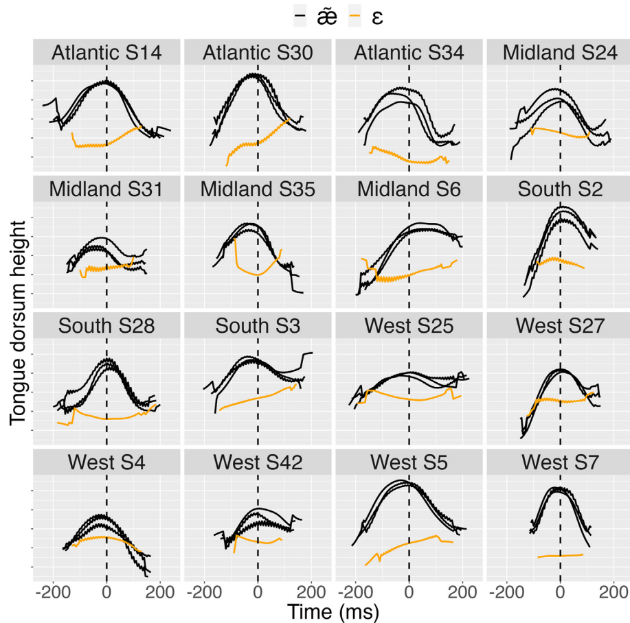
Fig. C1. Tongue dorsum trajectories aggregated for each of the 16 USE speakers separately for /æ/ before /n, nd, nz/ (black: three trajectories per speaker) and for /ε/ before /d/ (gold). The trajectories are based on the gridlines from the palatal region, with processing and normalization carried out as detailed in 2.5.2. Accordingly, all panels are scaled from 0 to 1 (1 corresponding to each speaker's most constricted dorsal tongue position). The regional affiliation (Appendix B) for each speaker is shown above each plot. The trajectories extend between the acoustic vowel onset and offset and were aggregated after alignment at the acoustic vowel midpoint (vertical dashed line).
