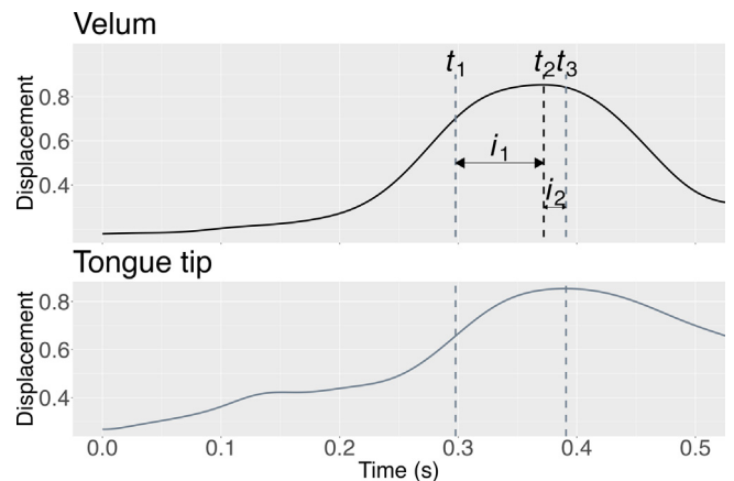
Fig. 11. Synchronized velum and tongue tip trajectories over a VN(C) interval. The times of the vertical dashed lines in row 1 are from left to right: ( t_1 ) peak velocity of tongue tip raising ( t_2 ) peak displacement of velum lowering ( t_3 ) peak displacement of tongue tip raising. The horizontal double arrows show the two parameters, i_1 and i_2 , that were analysed.
