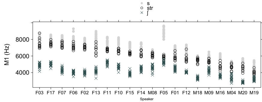
Fig. 3. Mean M1 for pre-vocalic sibilants /s, j/ and for the sibilant in /str/ produced by 20 speakers. One data point per sibilant token: light grey filled circles for /s/, dark grey crosses for /j/ and black open circles for /str/. Speakers are ordered along the x-axis in order of decreasing (mean) M1 in /str/.
