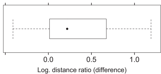
Fig. 5. The plot shows the difference (one value per speaker) between pre-vocalic and pre-consonantal /s/ on the log. distance ratio. Positive values indicate that the log. distance was greater for /s/ in pre-vocalic than in pre-consonantal position.
