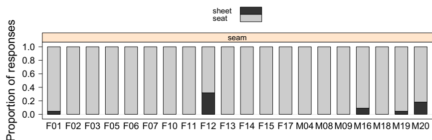
Fig. 8. Proportion of SHEET responses (in black) to sibilants in seam produced by twenty talkers (along the x-axis).
