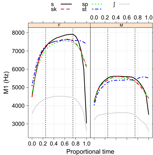
Fig. 4. First spectral moment trajectories during the sibilant in /sV/, /spV/, /stV/, /skV/ and /jV/ (where V=vowel). Tracks were averaged across speakers after averaging within context and speaker. The dotted vertical lines indicate the temporal middle half, over which mean M1 was calculated.
