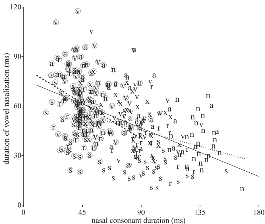
FIGURE 3. Scatter plot showing the inverse relation between nasal consonant duration and vowel nasalization duration for VNC_{\text{voiceless}} (circled letters) and VNC_{\text{voiced}} (plain letters) produced by six American English speakers. Letter type designates tokens from Speaker A, N, R, S, V, or X. Regression lines correspond to R^2 for each of the three statistical models described in the text (solid line = across contexts, dashed line = voiceless context, dotted line = voiced context).
