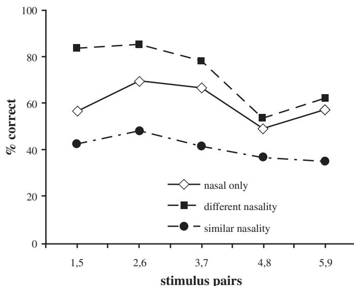
FIGURE 7. Pooled responses of twenty-seven American English-speaking listeners to three types of discrimination trials: nasal-only [gām s ba] – [gām l ba]), different nasality ([gā s m s ba] – [gā l m l ba]), and similar nasality ([gā l m s ba] – [gā s m l ba]).
