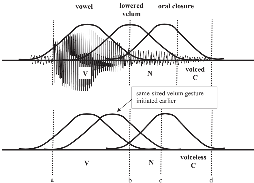
FIGURE 1. Schematic representation of the consequences for vowel nasalization, the nasal consonant, and the postnasal oral constriction if the velum gesture is initiated earlier in voiceless (bottom) than in voiced (top) contexts. Dashed lines indicate acoustic segmentation.
