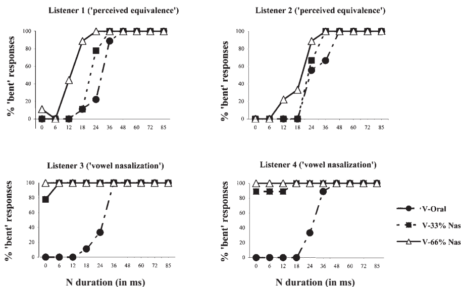
FIGURE 12. Percent ‘bent’ identification responses of four listeners (a subset of the original thirty listeners) to the bet – bent series for three degrees of vowel nasalization (shown by line type). Categorization as ‘perceived equivalence’ or ‘vowel nasalization’ listener is based on that listener’s discrimination judgments.
