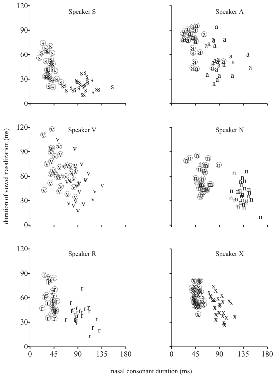
FIGURE 4. Scatter plot of the relation between nasal consonant duration and vowel nasalization duration for VNC voiceless (circled letters) and VNC voiced (plain letters) for each of the six speakers.
