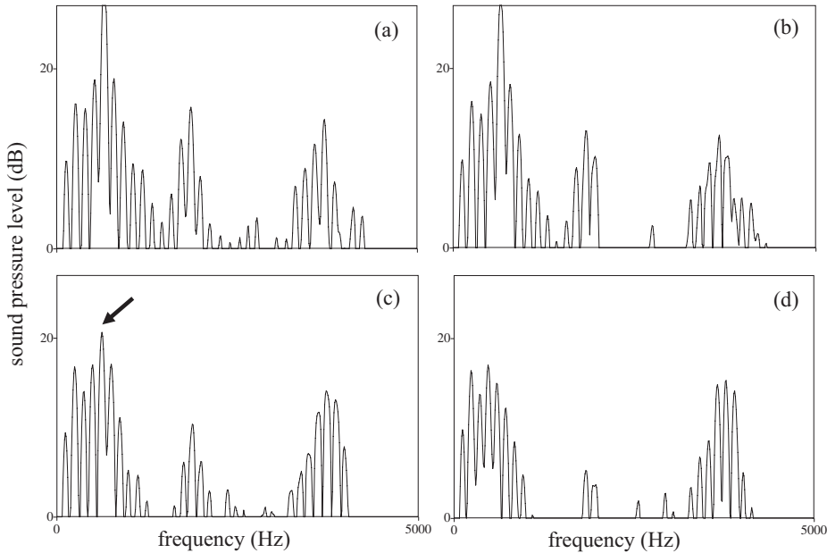
FIGURE 2. Four consecutive spectral sections (a–d) in 10 ms increments for [ɛ] from bent produced by a male speaker of American English. Onset of acoustic nasalization occurs in spectrum (c), where the arrow indicates reduced F1 amplitude (especially the fifth harmonic). Further flattening of the spectrum in the F1 region occurs as the vowel becomes more nasalized, as shown in spectrum (d).
