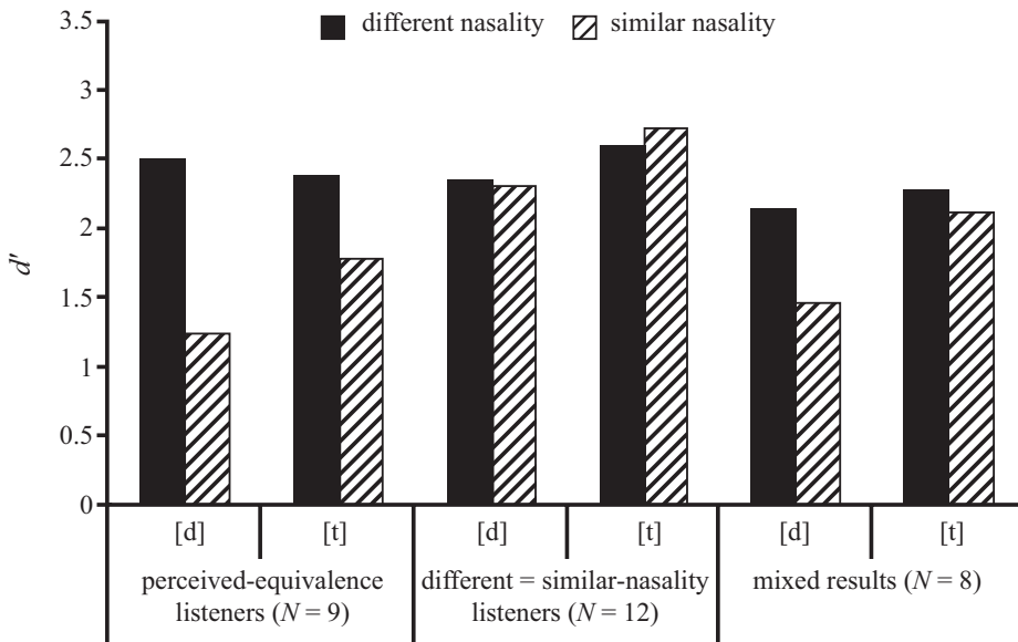
FIGURE 10. d' scores of three groups of listeners for the different- and similar-nasality trials, for two voicing contexts. See text for explanation of the listener groups.
