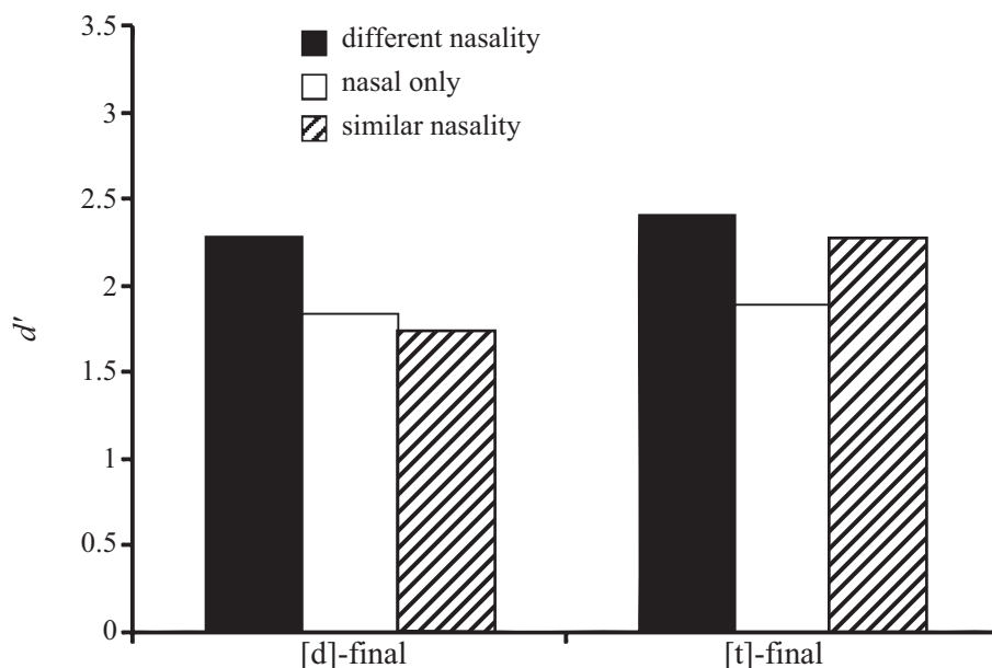
FIGURE 9. Pooled d' scores of thirty American English-speaking listeners for three types of discrimination trials in [d]-final and [t]-final contexts: nasal-only ( [\tilde{\epsilon}n_s] - [\tilde{\epsilon}n_L] ), different-nasality ( [\tilde{\epsilon}ns] - [\tilde{\epsilon}n_L] ), and similar-nasality ( [\tilde{\epsilon}_Ln_s] - [\tilde{\epsilon}_sn_L] ). All pairwise comparisons within a voicing context were significant except that the nasal-only – similar-nasality comparison was not significant for [d]-final stimuli, nor was the different-nasality – similar-nasality comparison significant for [t]-final stimuli.
