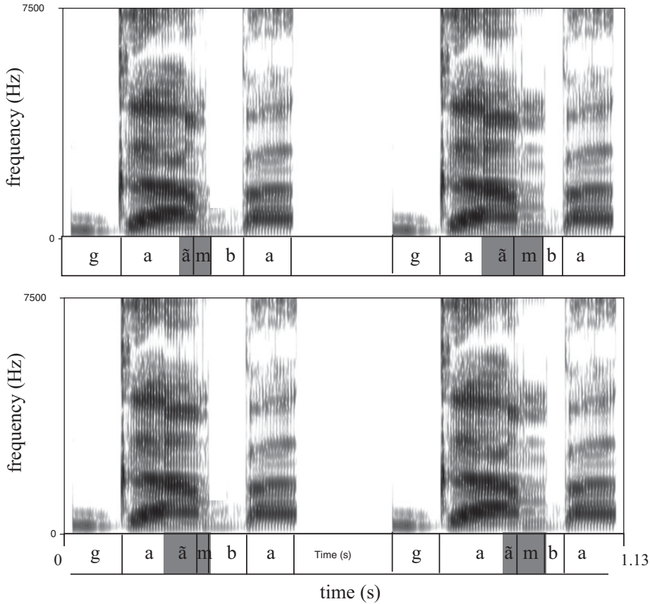
FIGURE 6. Illustrative different-nasality (top) and similar-nasality (bottom) pairs. The shaded portions of the transcription grids indicate the nasal ( \tilde{V} and N) portion of each pair member.
