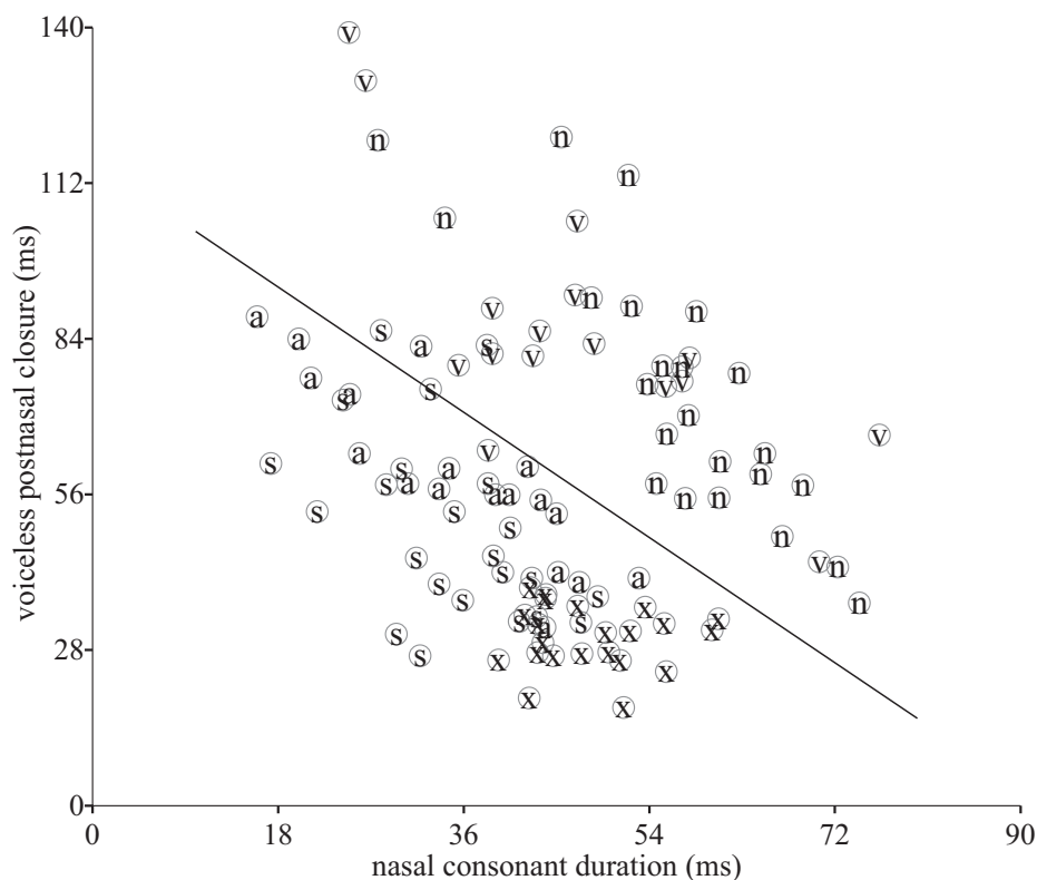
FIGURE 5. Scatter plot showing the inverse relation between nasal consonant duration and duration of postnasal oral closure for words with /Vnt/ sequences produced by Speakers A, N, S, V, and X. Regression line corresponds to R^2 from the statistical model described in the text.
