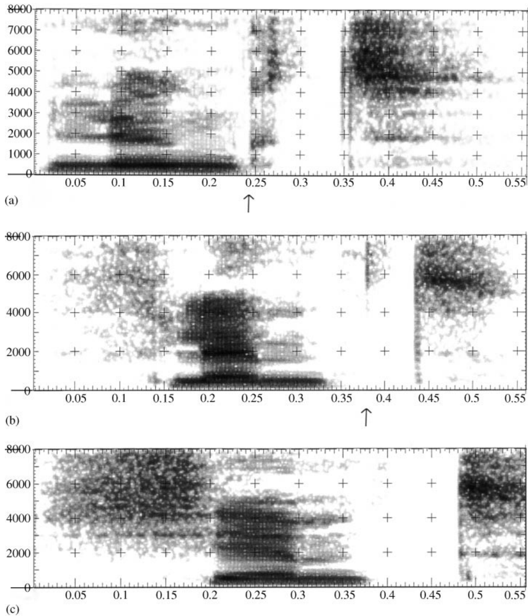
Figure 1. Spectrograms of an item with a strong epenthetic burst (/lyŋt/ [lyŋkt] 1(a)), a weak epenthetic burst (/flemt/ [flemt] 1(b)), and no visible epenthetic burst (/femt/ [femt] 1(c)). In 1a and 1b, the arrow marks the beginning of the epenthetic burst.
