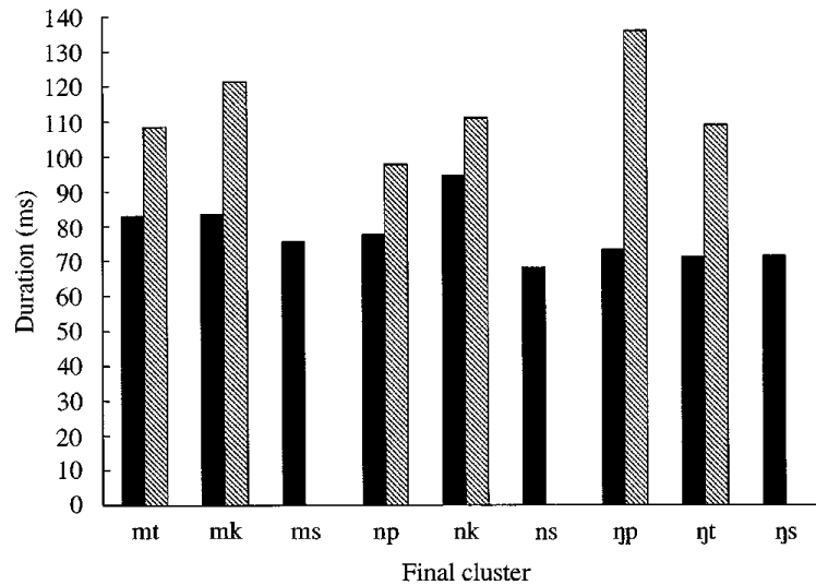
Figure 10. Average duration of nasal and average duration of entire closure from end of nasal voicing to beginning of intended stop burst, by cluster, for all stimulus items. Closure duration not included for clusters ending in /s/. ■ nasal; ▨ total stop closure.
