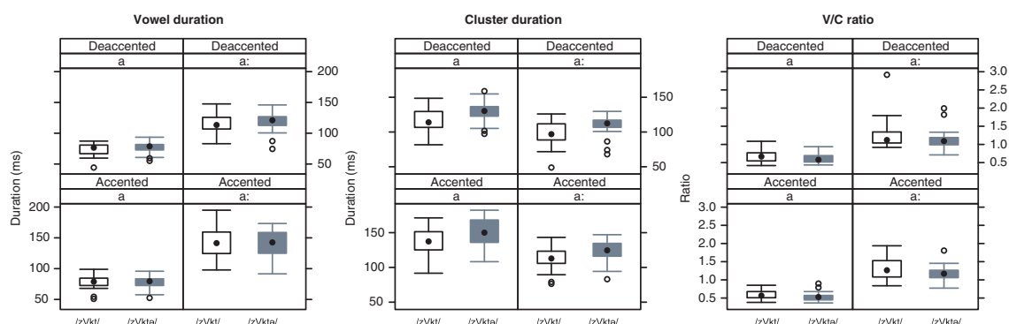
Figure 14: Mean durations of the vowel (left), of the following /kt/ cluster (center), and the ratio between the two (right) shown separately for stress (accented/deaccented), tensity (/a, a:/), and syllable count (white/grey rectangles for monosyllabic/disyllabic). The data were aggregated by speaker so that each boxplot includes one data point per speaker. The extent of the rectangle is the interquartile range.
