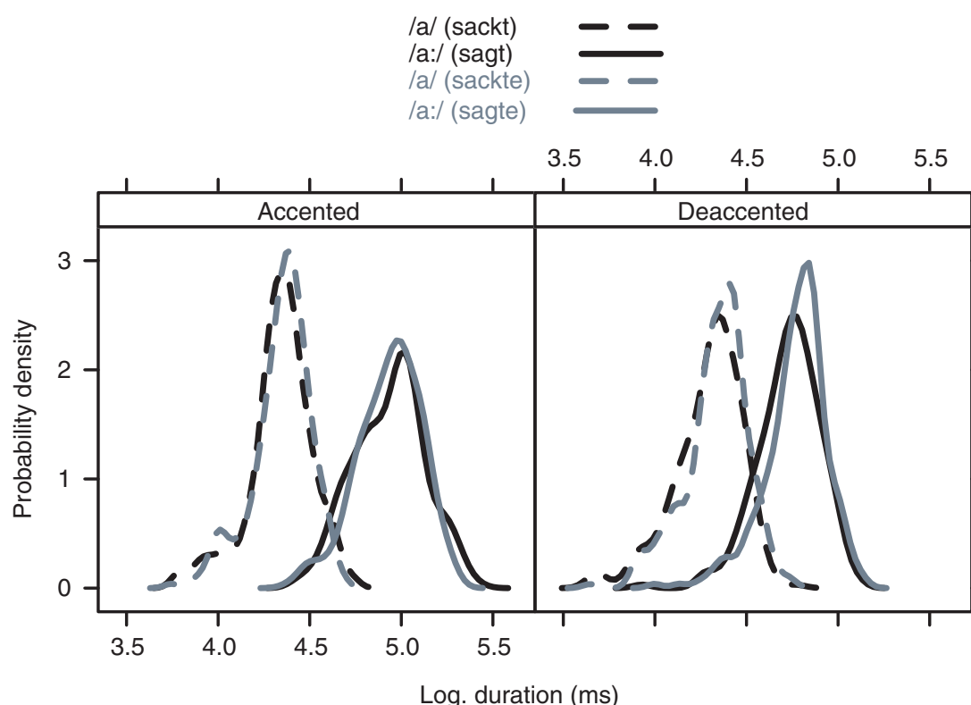
Figure 2: Probability density plots of the log vowel duration for all samples of the corpus in monosyllabic (black) and disyllabic (grey) words in accented (left) and deaccented (right) contexts for tense (solid) and lax (dashed) categories.
