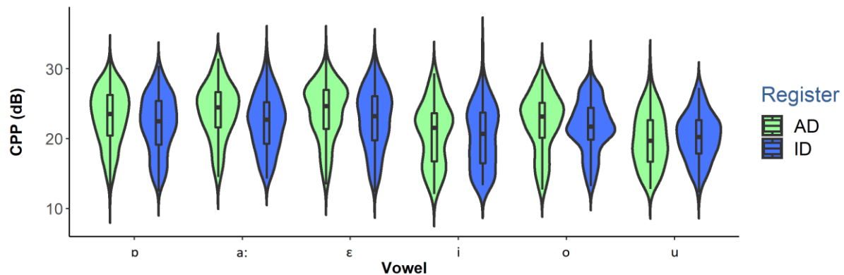
Figure 1. CPP values for each investigated vowel in the two registers.
